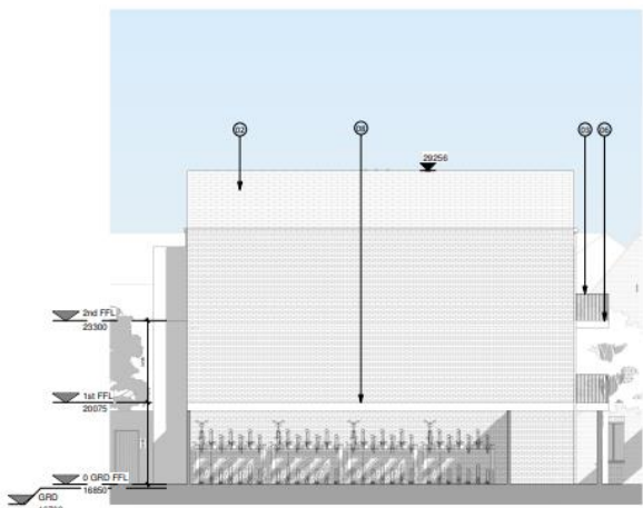
① 2006 - North Elevation (Block B) 1 : 100
