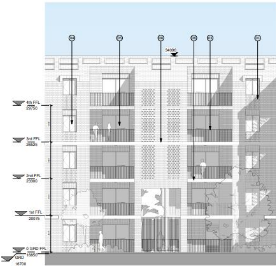
3 2004 - West Courtyard Elevation (Block A) 1 : 100
