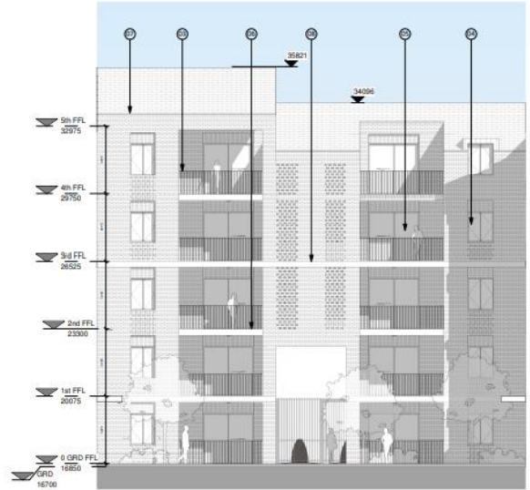
4 2004 - East Courtyard Elevation (Block A) 1 : 100
